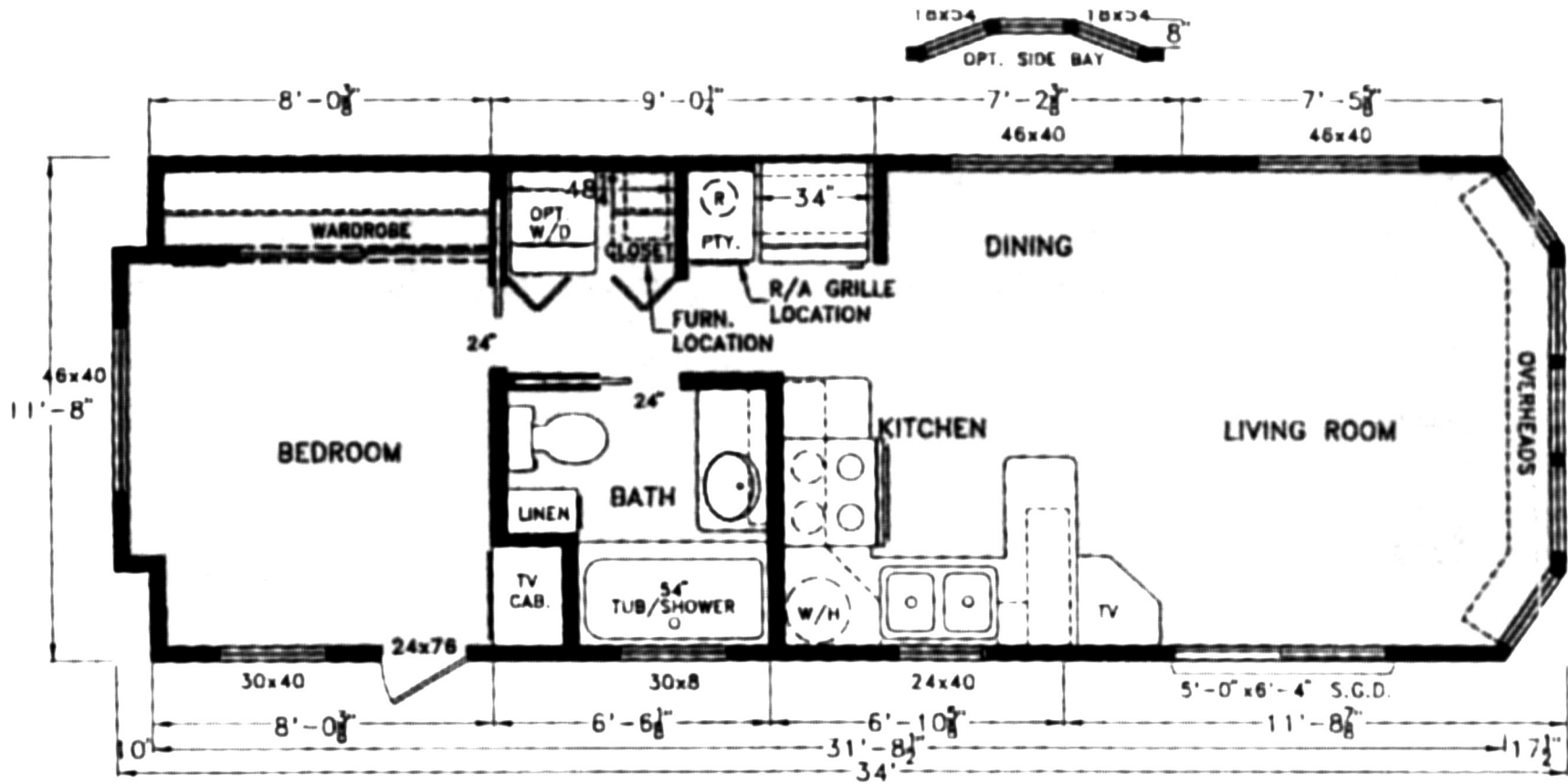
one bedroom Model 448-34'0"
