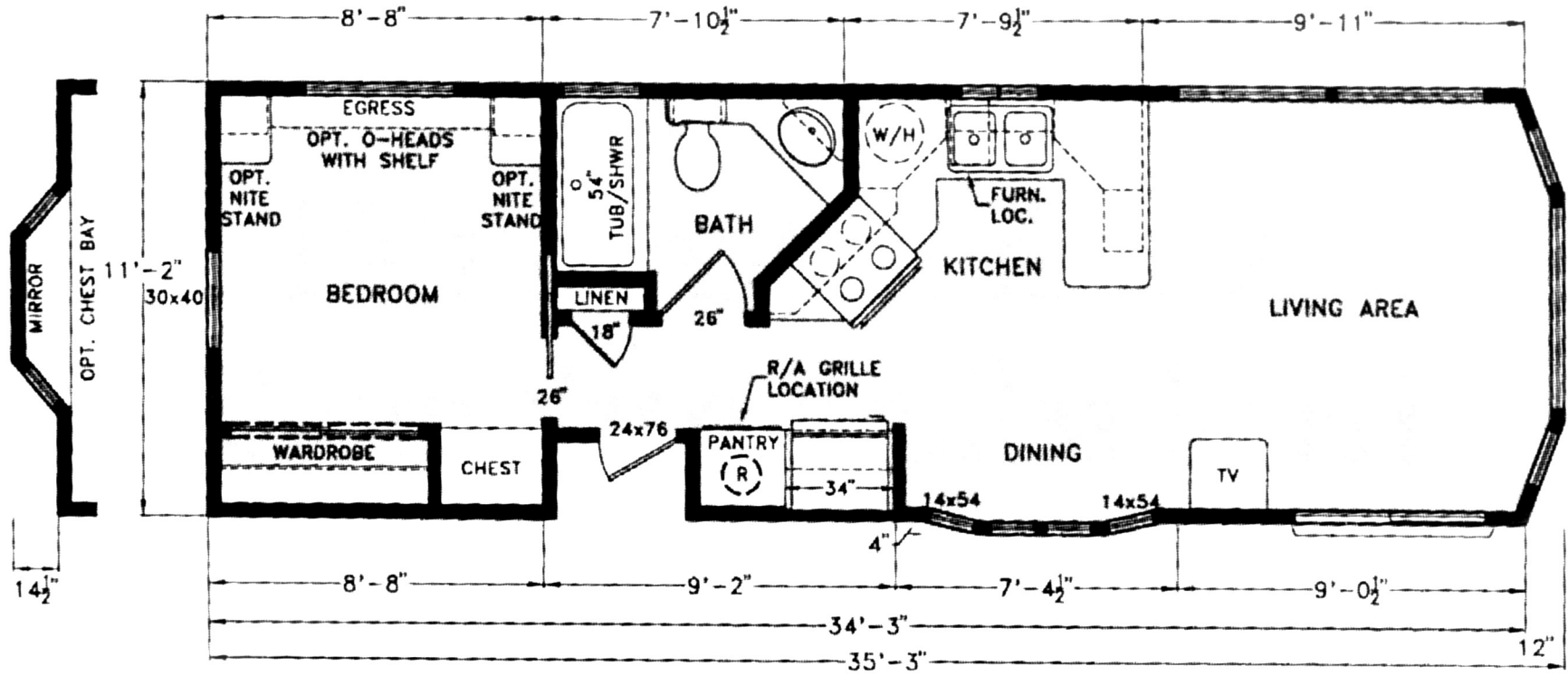
MODEL: 447-35'3"
